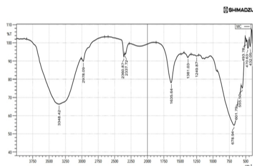
Graph.2. FT-IR spectrum of chitin silver nanoparticles
